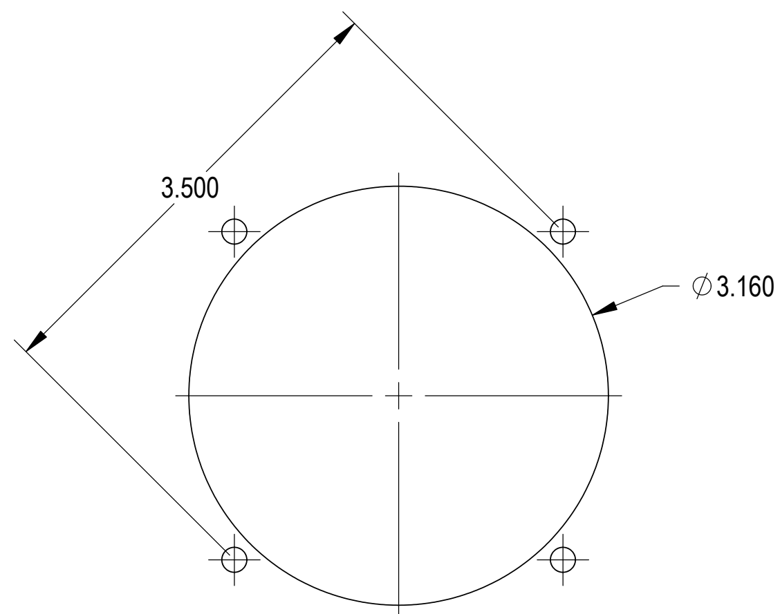
STANDARD INSTRUMENT CUT-OUT
