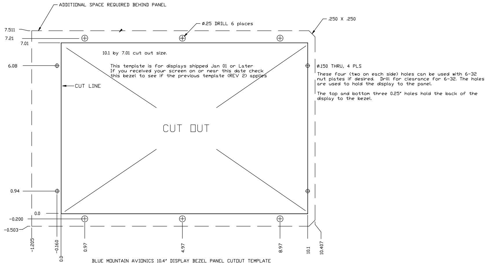
BLUE MOUNTAIN AVIONICS 10.4' DISPLAY BEZEL PANEL CUTOUT TEMPLATE
